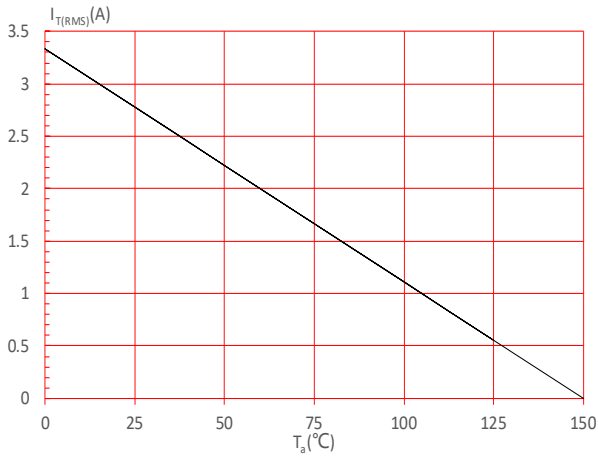
FIG.5: On-state characteristics
