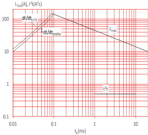
FIG.6: Non-repetitive surge peak on-state current for a sinusoidal pulse with width t_p < 20\text{ms} , and corresponding value of I^2t ( I - II : di/dt < 50\text{A}/\mu\text{s} ; III-IV : di/dt < 30\text{A}/\mu\text{s} )
