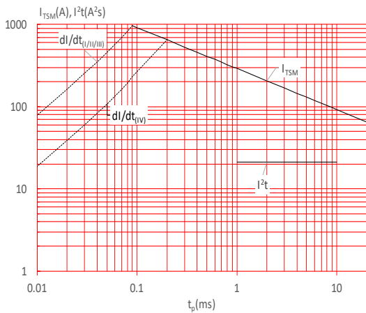
FIG.5: Non-repetitive surge peak on-state current for a sinusoidal pulse with width t_p < 20\text{ms} , and corresponding value of I^2t ( I -II -III: di/dt < 80\text{A}/\mu\text{s} ; IV: di/dt < 40\text{A}/\mu\text{s} )
