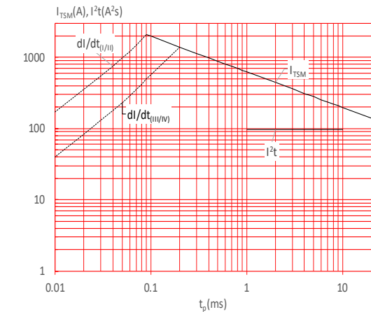
FIG.6: Non-repetitive surge peak on-state current for a sinusoidal pulse with width t_p < 20\text{ms} , and corresponding value of I^2t (I - II: di/dt < 80\text{A}/\mu\text{s} ; III-IV: di/dt < 50\text{A}/\mu\text{s} )
